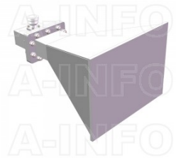
LB-284-15-C-7/16FSPO Standard Gain Horn Antenna 2.6-3.95GHz 15dB Gain 7/16(DIN) Female
